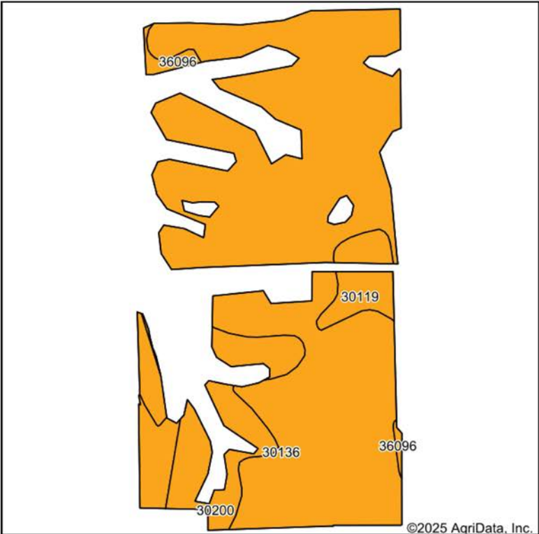
Daviness 80 Soils map
